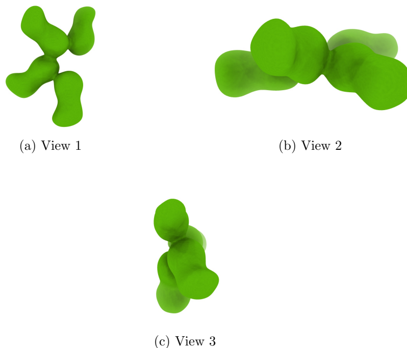
Figure 4: Isosurface at threshold=0.761000. Views generated by ChimeraX at a the following X, Y, Z angles: View 1 (0, -90, -90), View 2 (-90, 0, -90), View 3 (0, 0, 0).
