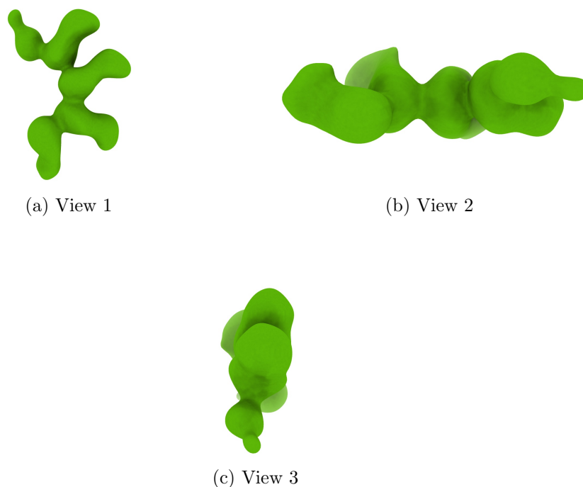
Figure 4: Isosurface at threshold=0.908000. Views generated by ChimeraX at a the following X, Y, Z angles: View 1 (0, -90, -90), View 2 (-90, 0, -90), View 3 (0, 0, 0).
