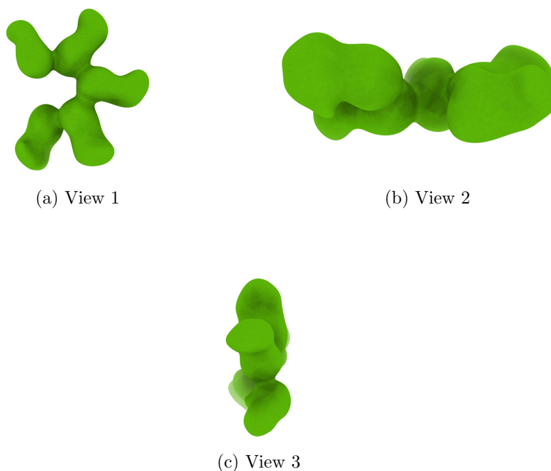
Figure 4: Isosurface at threshold=0.704000. Views generated by ChimeraX at a the following X, Y, Z angles: View 1 (0, -90, -90), View 2 (-90, 0, -90), View 3 (0, 0, 0).
