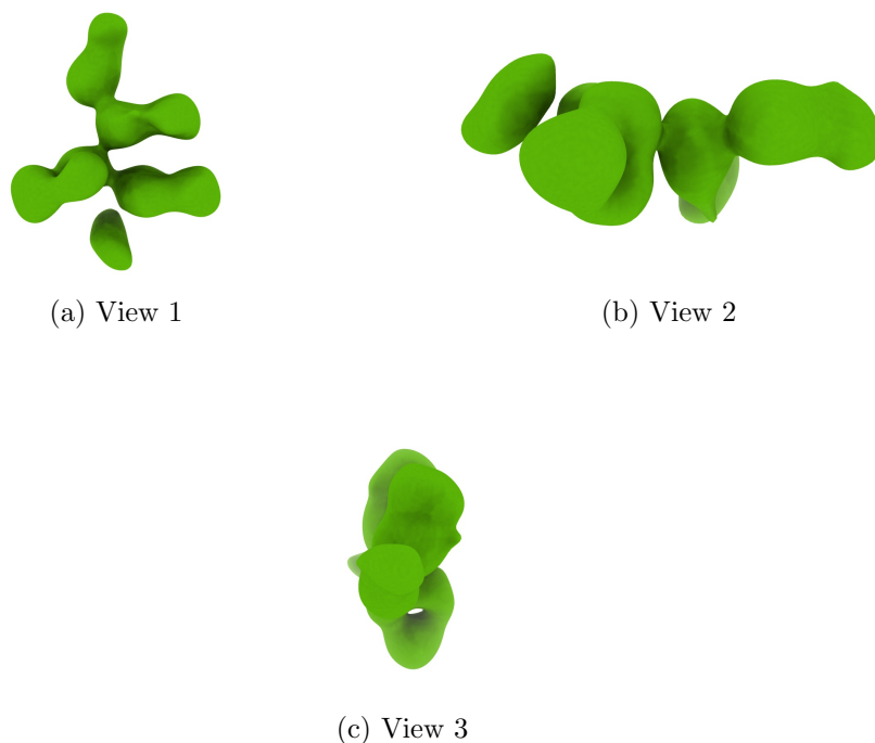
Figure 4: Isosurface at threshold=0.934000. Views generated by ChimeraX at a the following X, Y, Z angles: View 1 (0, -90, -90), View 2 (-90, 0, -90), View 3 (0, 0, 0).
