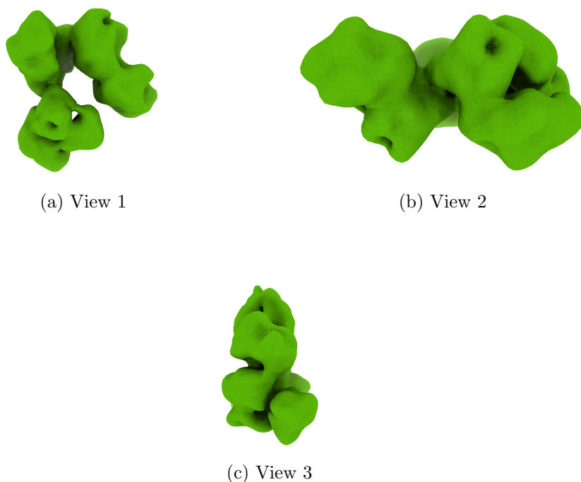
Figure 4: Isosurface at threshold=1.400000. Views generated by ChimeraX at a the following X, Y, Z angles: View 1 (0, -90, -90), View 2 (-90, 0, -90), View 3 (0, 0, 0).
