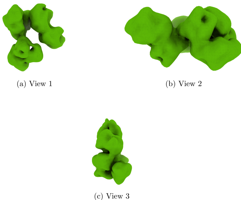
Figure 4: Isosurface at threshold=1.400000. Views generated by ChimeraX at the following X, Y, Z angles: View 1 (0, -90, -90), View 2 (-90, 0, -90), View 3 (0, 0, 0).
