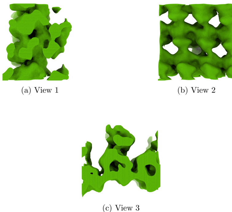
Figure 4: Isosurface at threshold=1.340000. Views generated by ChimeraX at a the following X, Y, Z angles: View 1 (0, -90, -90), View 2 (-90, 0, -90), View 3 (0, 0, 0).
