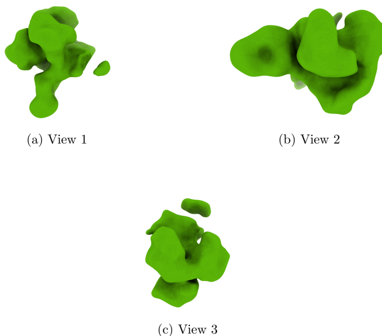
Figure 4: Isosurface at threshold=0.530000. Views generated by ChimeraX at a the following X, Y, Z angles: View 1 (0, -90, -90), View 2 (-90, 0, -90), View 3 (0, 0, 0).
