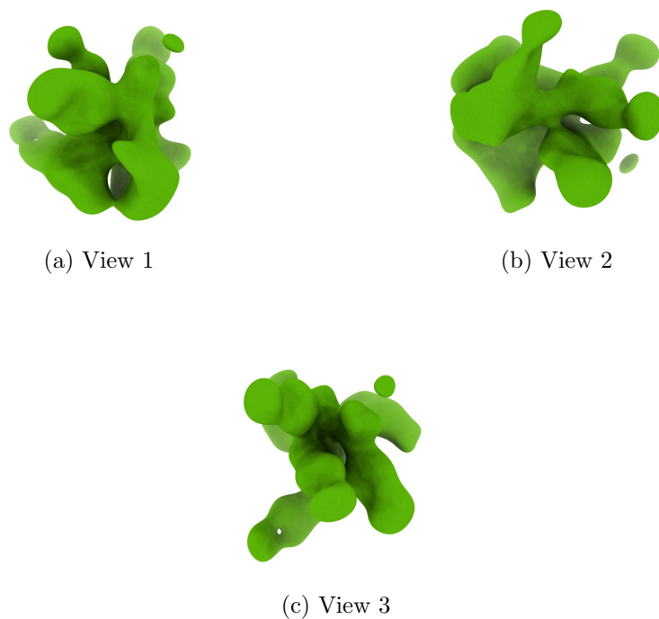
Figure 4: Isosurface at threshold=0.019000. Views generated by ChimeraX at a the following X, Y, Z angles: View 1 (0, -90, -90), View 2 (-90, 0, -90), View 3 (0, 0, 0).
