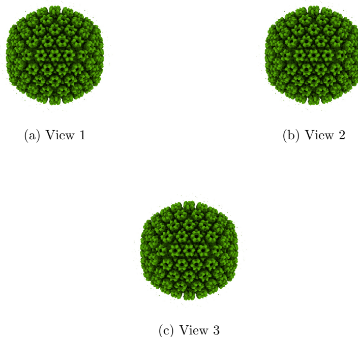
Figure 4: Isosurface at threshold=1450.000000. Views generated by ChimeraX at the following X, Y, Z angles: View 1 (0, -90, -90), View 2 (-90, 0, -90), View 3 (0, 0, 0).
