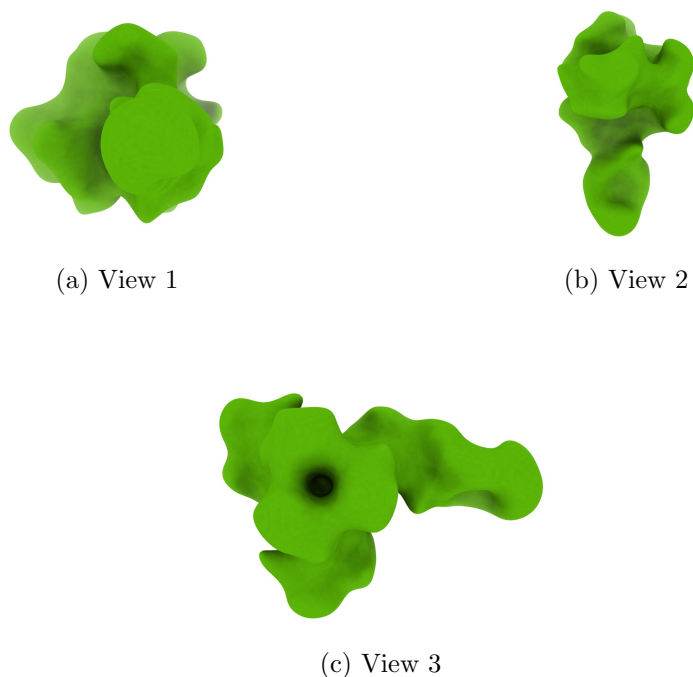
Figure 4: Isosurface at threshold=0.015000. Views generated by ChimeraX at the following X, Y, Z angles: View 1 (0, -90, -90), View 2 (-90, 0, -90), View 3 (0, 0, 0).
