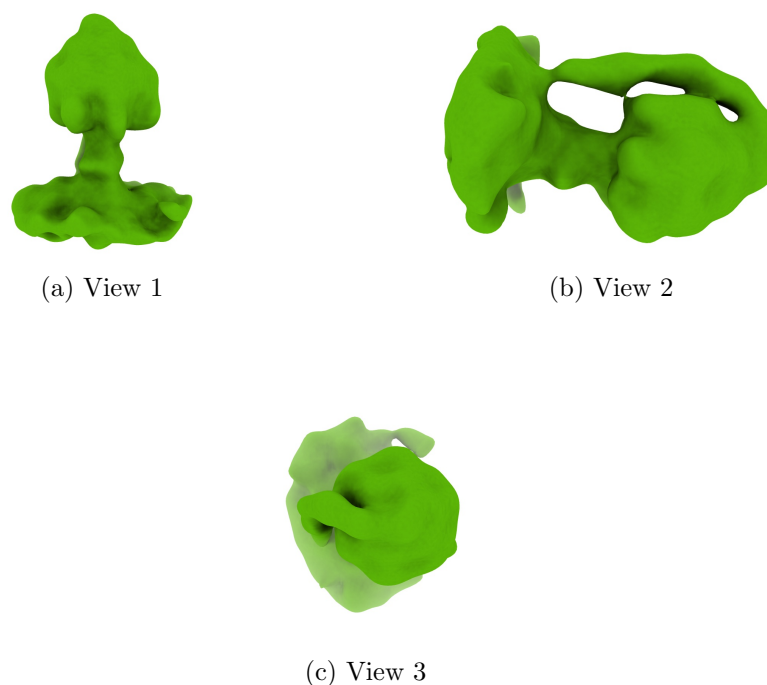
Figure 4: Isosurface at threshold=0.022500. Views generated by ChimeraX at a the following X, Y, Z angles: View 1 (0, -90, -90), View 2 (-90, 0, -90), View 3 (0, 0, 0).
