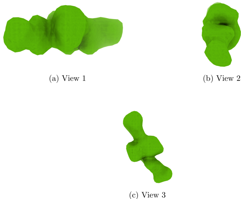
Figure 4: Isosurface at threshold=4.890000. Views generated by ChimeraX at a the following X, Y, Z angles: View 1 (0, -90, -90), View 2 (-90, 0, -90), View 3 (0, 0, 0).
