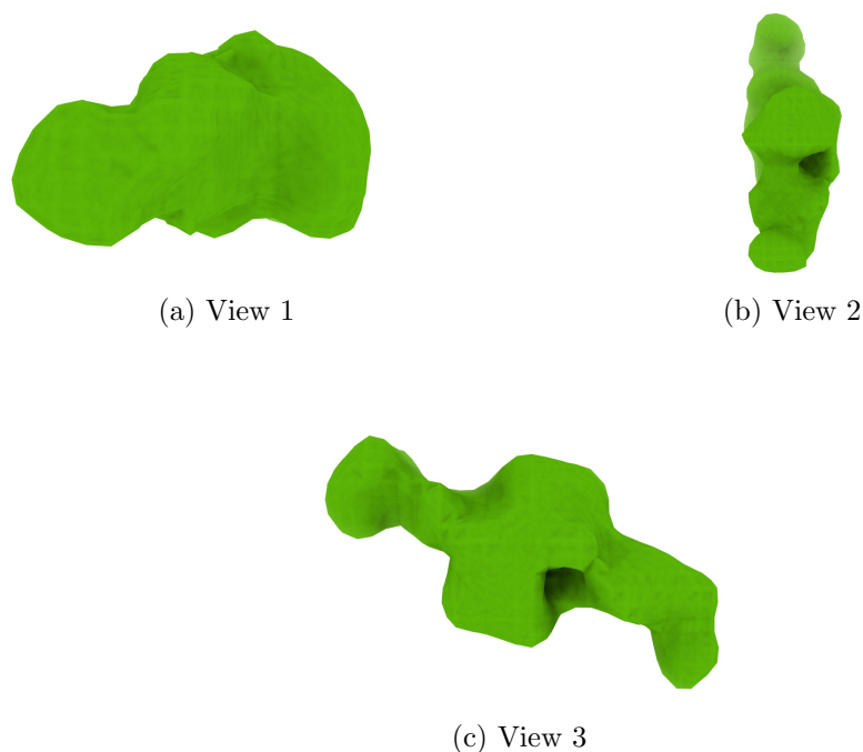
Figure 4: Isosurface at threshold=5.110000. Views generated by ChimeraX at a the following X, Y, Z angles: View 1 (0, -90, -90), View 2 (-90, 0, -90), View 3 (0, 0, 0).
