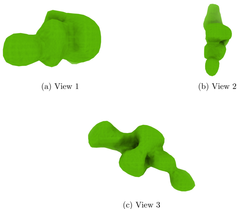
Figure 4: Isosurface at threshold=5.380000. Views generated by ChimeraX at a the following X, Y, Z angles: View 1 (0, -90, -90), View 2 (-90, 0, -90), View 3 (0, 0, 0).
