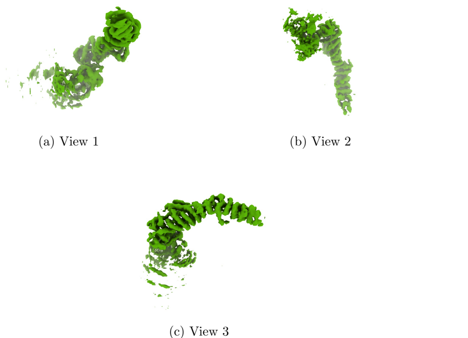
Figure 4: Isosurface at threshold=0.014400. Views generated by ChimeraX at a the following X, Y, Z angles: View 1 (0, -90, -90), View 2 (-90, 0, -90), View 3 (0, 0, 0).
