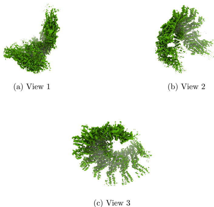
Figure 4: Isosurface at threshold=0.019800. Views generated by ChimeraX at a the following X, Y, Z angles: View 1 (0, -90, -90), View 2 (-90, 0, -90), View 3 (0, 0, 0).
