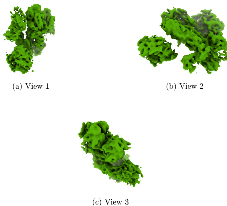
Figure 4: Isosurface at threshold=0.009710. Views generated by ChimeraX at a the following X, Y, Z angles: View 1 (0, -90, -90), View 2 (-90, 0, -90), View 3 (0, 0, 0).
