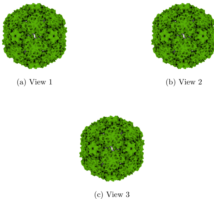
Figure 4: Isosurface at threshold=1.370000. Views generated by ChimeraX at a the following X, Y, Z angles: View 1 (0, -90, -90), View 2 (-90, 0, -90), View 3 (0, 0, 0).
