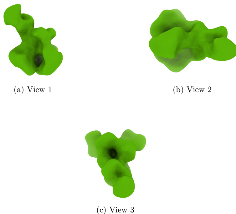
Figure 4: Isosurface at threshold=0.018000. Views generated by ChimeraX at the following X, Y, Z angles: View 1 (0, -90, -90), View 2 (-90, 0, -90), View 3 (0, 0, 0).
