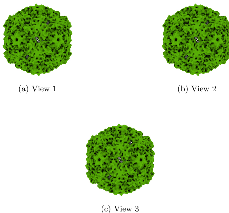
Figure 4: Isosurface at threshold=1.530000. Views generated by ChimeraX at a the following X, Y, Z angles: View 1 (0, -90, -90), View 2 (-90, 0, -90), View 3 (0, 0, 0).
