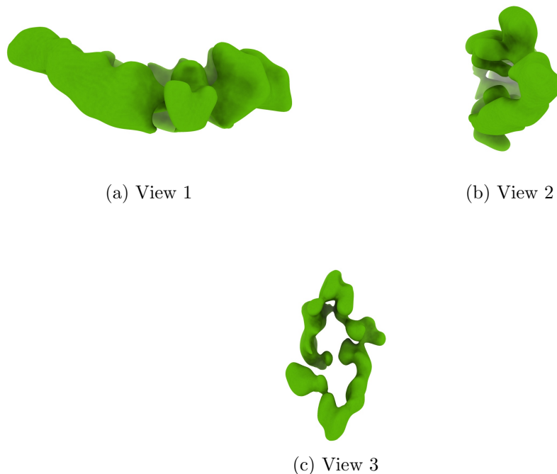
Figure 4: Isosurface at threshold=0.006300. Views generated by ChimeraX at a the following X, Y, Z angles: View 1 (0, -90, -90), View 2 (-90, 0, -90), View 3 (0, 0, 0).
