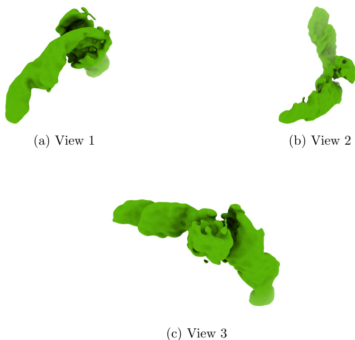
Figure 4: Isosurface at threshold=0.008100. Views generated by ChimeraX at a the following X, Y, Z angles: View 1 (0, -90, -90), View 2 (-90, 0, -90), View 3 (0, 0, 0).
