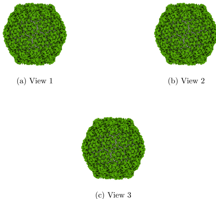
Figure 4: Isosurface at threshold=4.800000. Views generated by ChimeraX at a the following X, Y, Z angles: View 1 (0, -90, -90), View 2 (-90, 0, -90), View 3 (0, 0, 0).
