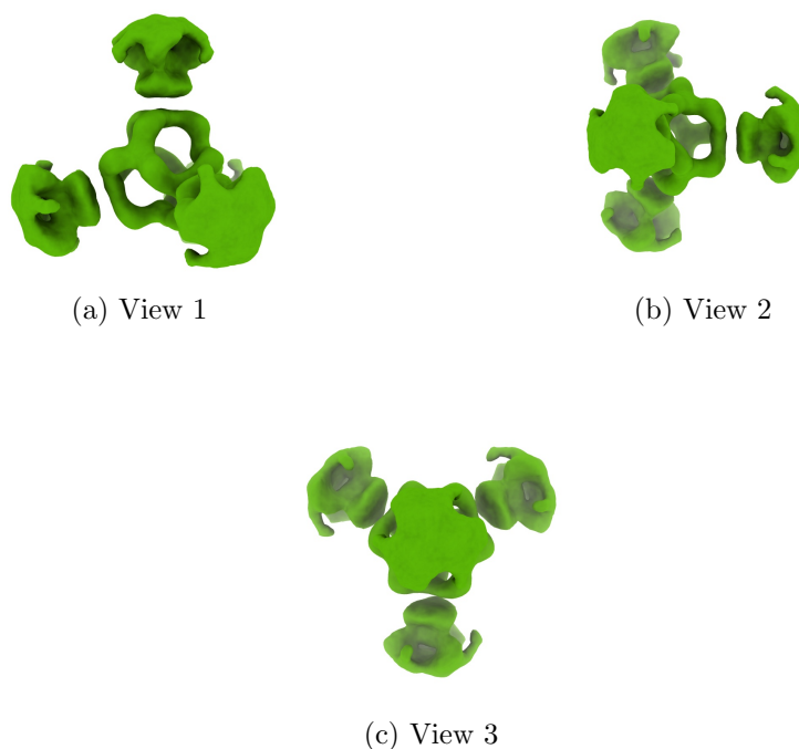
Figure 4: Isosurface at threshold=0.024000. Views generated by ChimeraX at a the following X, Y, Z angles: View 1 (0, -90, -90), View 2 (-90, 0, -90), View 3 (0, 0, 0).
