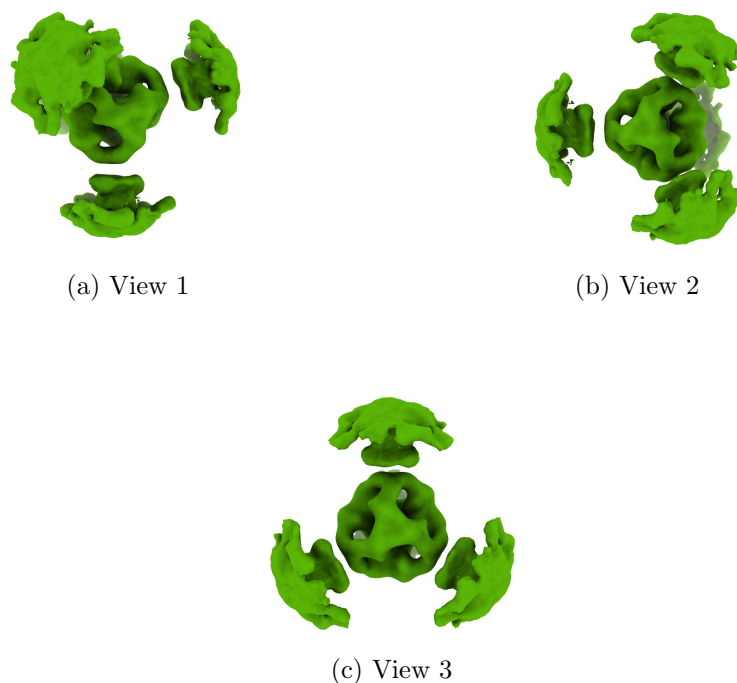
Figure 4: Isosurface at threshold=0.005500. Views generated by ChimeraX at a the following X, Y, Z angles: View 1 (0, -90, -90), View 2 (-90, 0, -90), View 3 (0, 0, 0).
