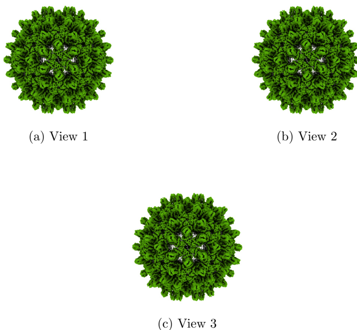
Figure 4: Isosurface at threshold=0.049300. Views generated by ChimeraX at a the following X, Y, Z angles: View 1 (0, -90, -90), View 2 (-90, 0, -90), View 3 (0, 0, 0).
