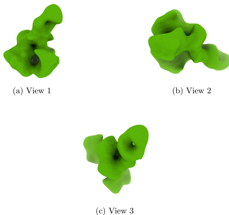
Figure 4: Isosurface at threshold=0.020000. Views generated by ChimeraX at the following X, Y, Z angles: View 1 (0, -90, -90), View 2 (-90, 0, -90), View 3 (0, 0, 0).
