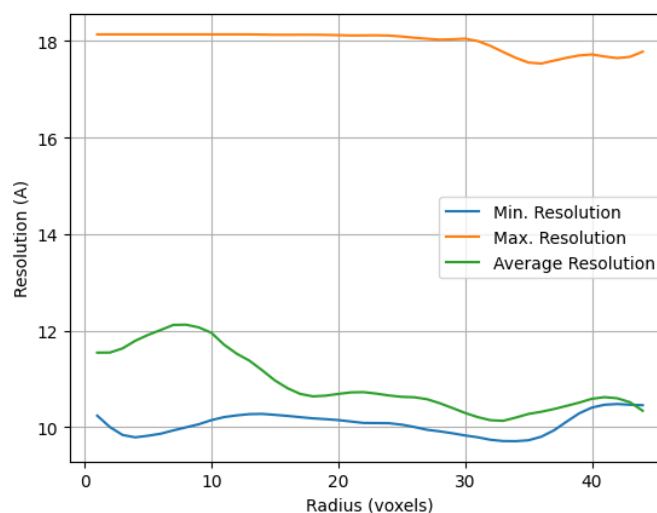
Figure 23: Radial averages (in space) of the minimum, maximum and average resolution at each voxel.
