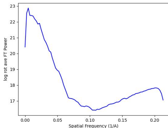
Figure 30: Logarithm of the radial average of the input map power in Fourier space.
