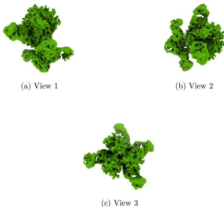
Figure 4: Isosurface at threshold=0.019800. Views generated by ChimeraX at a the following X, Y, Z angles: View 1 (0, -90, -90), View 2 (-90, 0, -90), View 3 (0, 0, 0).
