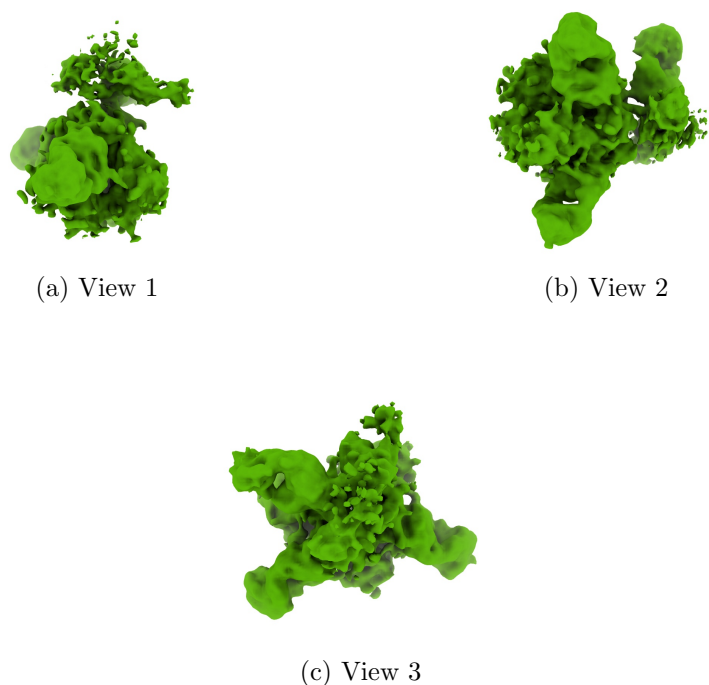
Figure 4: Isosurface at threshold=0.008270. Views generated by ChimeraX at a the following X, Y, Z angles: View 1 (0, -90, -90), View 2 (-90, 0, -90), View 3 (0, 0, 0).
