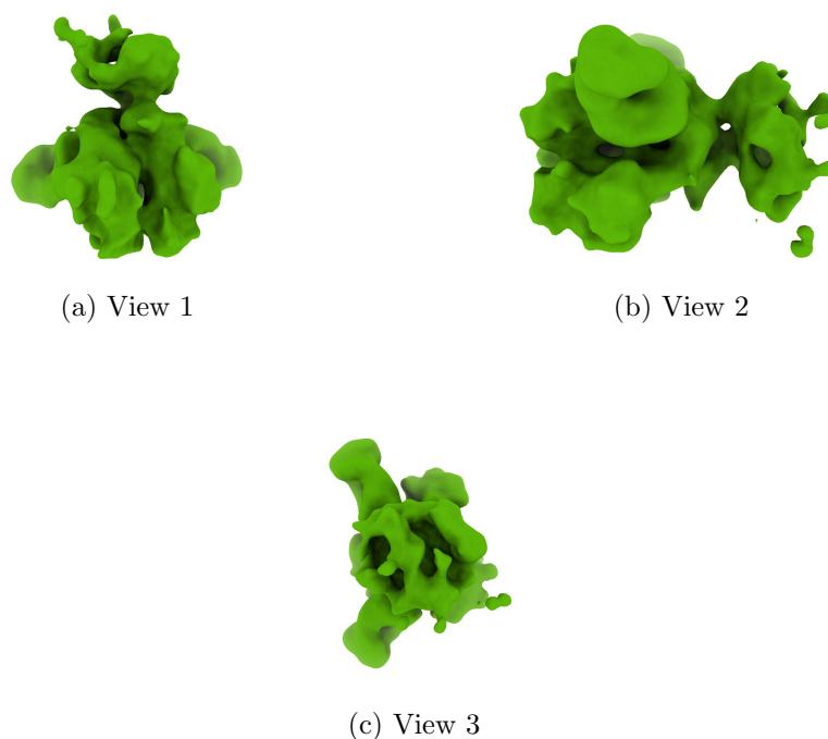
Figure 4: Isosurface at threshold=0.224000. Views generated by ChimeraX at a the following X, Y, Z angles: View 1 (0, -90, -90), View 2 (-90, 0, -90), View 3 (0, 0, 0).
