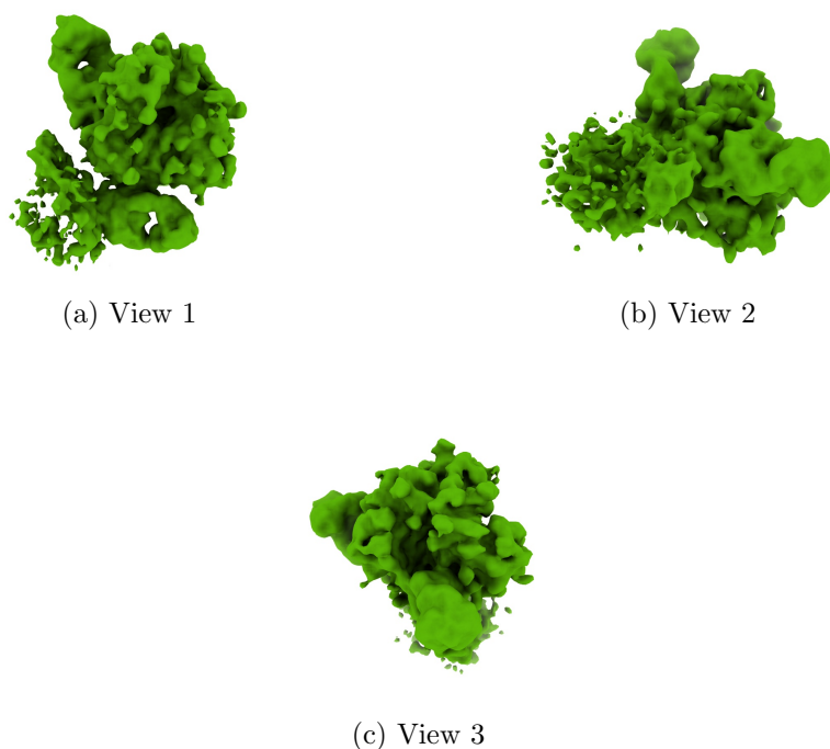
Figure 4: Isosurface at threshold=0.217000. Views generated by ChimeraX at a the following X, Y, Z angles: View 1 (0, -90, -90), View 2 (-90, 0, -90), View 3 (0, 0, 0).
