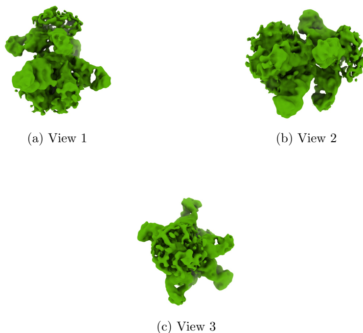
Figure 4: Isosurface at threshold=0.014800. Views generated by ChimeraX at a the following X, Y, Z angles: View 1 (0, -90, -90), View 2 (-90, 0, -90), View 3 (0, 0, 0).
