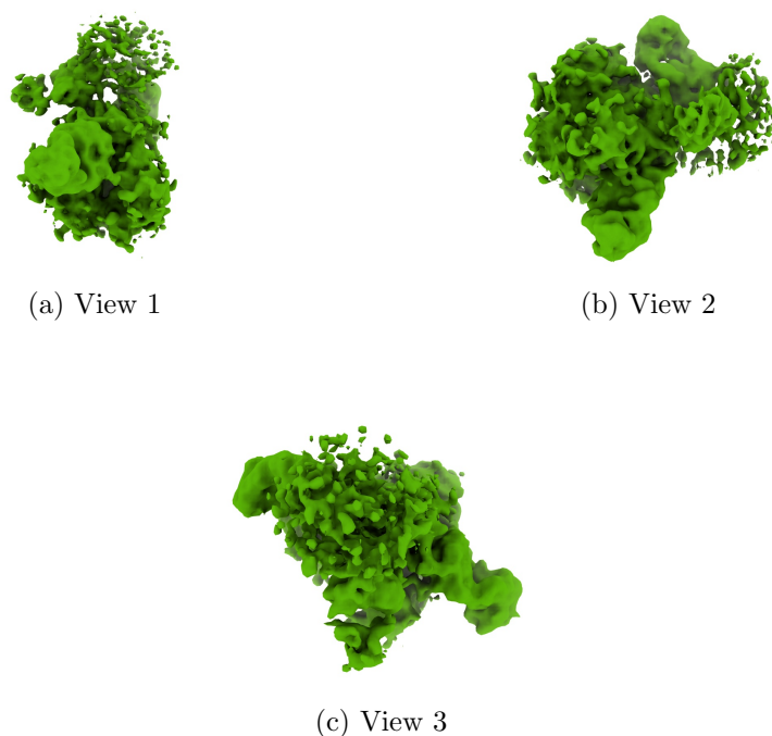
Figure 4: Isosurface at threshold=0.014500. Views generated by ChimeraX at a the following X, Y, Z angles: View 1 (0, -90, -90), View 2 (-90, 0, -90), View 3 (0, 0, 0).
