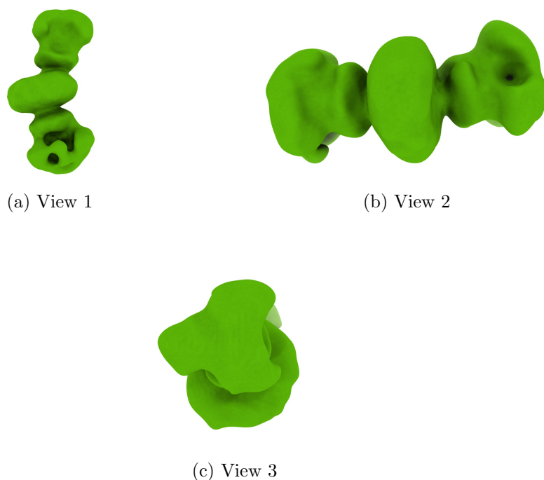
Figure 4: Isosurface at threshold=0.827000. Views generated by ChimeraX at a the following X, Y, Z angles: View 1 (0, -90, -90), View 2 (-90, 0, -90), View 3 (0, 0, 0).
