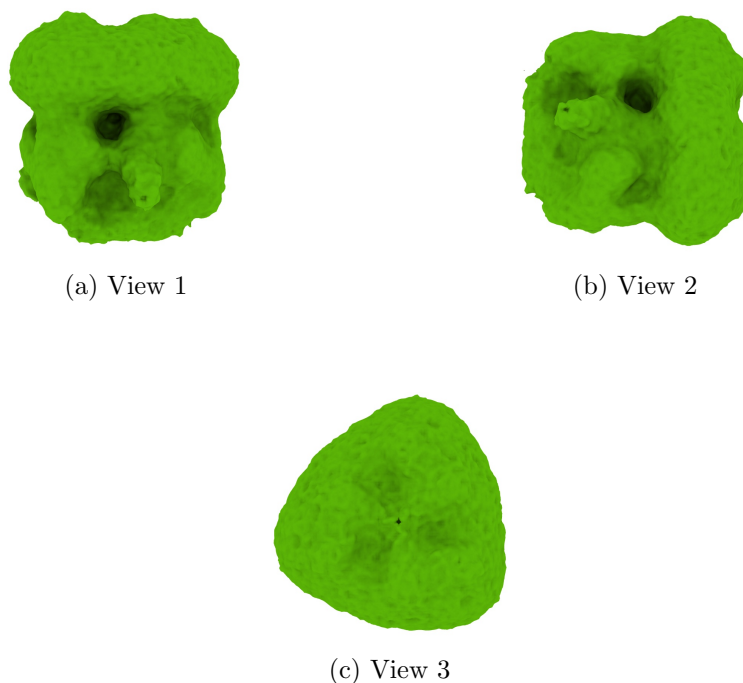
Figure 4: Isosurface at threshold=0.053900. Views generated by ChimeraX at a the following X, Y, Z angles: View 1 (0, -90, -90), View 2 (-90, 0, -90), View 3 (0, 0, 0).
