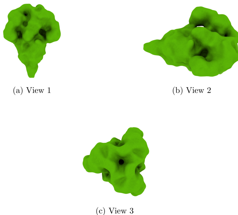
Figure 4: Isosurface at threshold=0.840000. Views generated by ChimeraX at a the following X, Y, Z angles: View 1 (0, -90, -90), View 2 (-90, 0, -90), View 3 (0, 0, 0).
