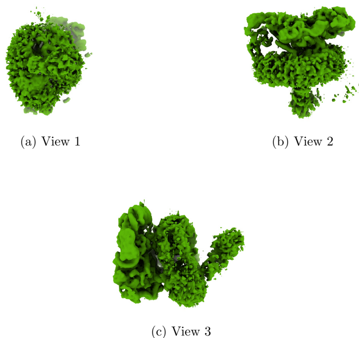
Figure 4: Isosurface at threshold=0.009500. Views generated by ChimeraX at a the following X, Y, Z angles: View 1 (0, -90, -90), View 2 (-90, 0, -90), View 3 (0, 0, 0).
