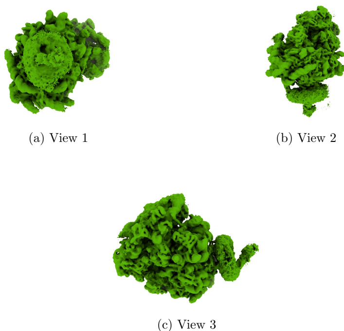
Figure 4: Isosurface at threshold=0.007300. Views generated by ChimeraX at a the following X, Y, Z angles: View 1 (0, -90, -90), View 2 (-90, 0, -90), View 3 (0, 0, 0).
