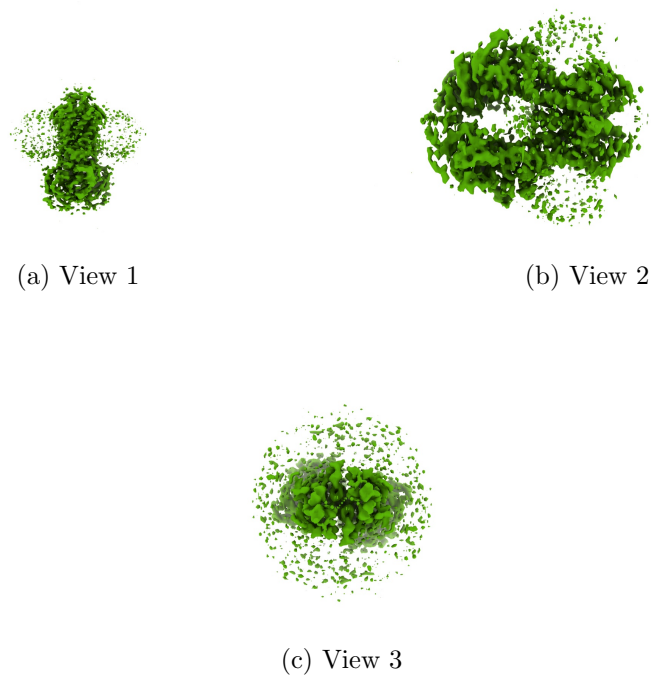
Figure 4: Isosurface at threshold=0.065000. Views generated by ChimeraX at a the following X, Y, Z angles: View 1 (0, -90, -90), View 2 (-90, 0, -90), View 3 (0, 0, 0).
