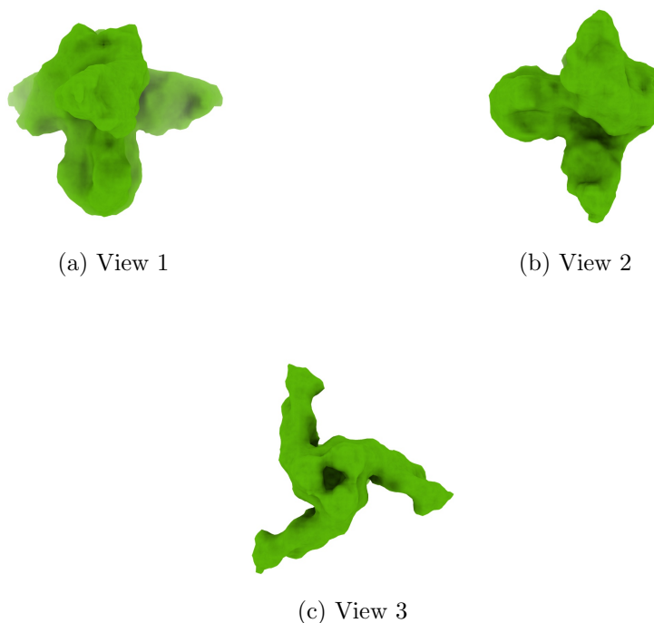
Figure 4: Isosurface at threshold=4.800000. Views generated by ChimeraX at a the following X, Y, Z angles: View 1 (0, -90, -90), View 2 (-90, 0, -90), View 3 (0, 0, 0).
