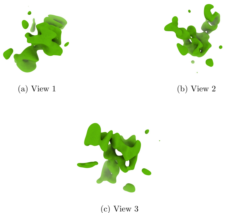
Figure 4: Isosurface at threshold=0.013600. Views generated by ChimeraX at a the following X, Y, Z angles: View 1 (0, -90, -90), View 2 (-90, 0, -90), View 3 (0, 0, 0).
