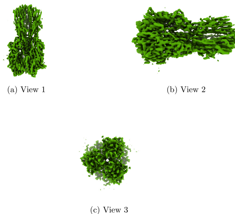
Figure 4: Isosurface at threshold=0.932000. Views generated by ChimeraX at a the following X, Y, Z angles: View 1 (0, -90, -90), View 2 (-90, 0, -90), View 3 (0, 0, 0).
