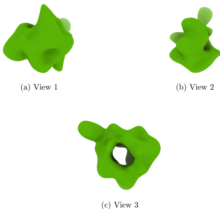
Figure 4: Isosurface at threshold=2.500000. Views generated by ChimeraX at a the following X, Y, Z angles: View 1 (0, -90, -90), View 2 (-90, 0, -90), View 3 (0, 0, 0).
