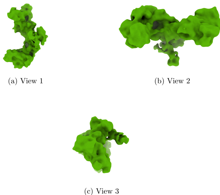
Figure 4: Isosurface at threshold=0.014200. Views generated by ChimeraX at a the following X, Y, Z angles: View 1 (0, -90, -90), View 2 (-90, 0, -90), View 3 (0, 0, 0).
