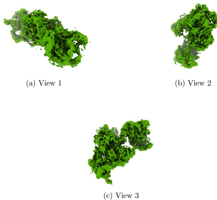
Figure 4: Isosurface at threshold=0.037400. Views generated by ChimeraX at a the following X, Y, Z angles: View 1 (0, -90, -90), View 2 (-90, 0, -90), View 3 (0, 0, 0).
