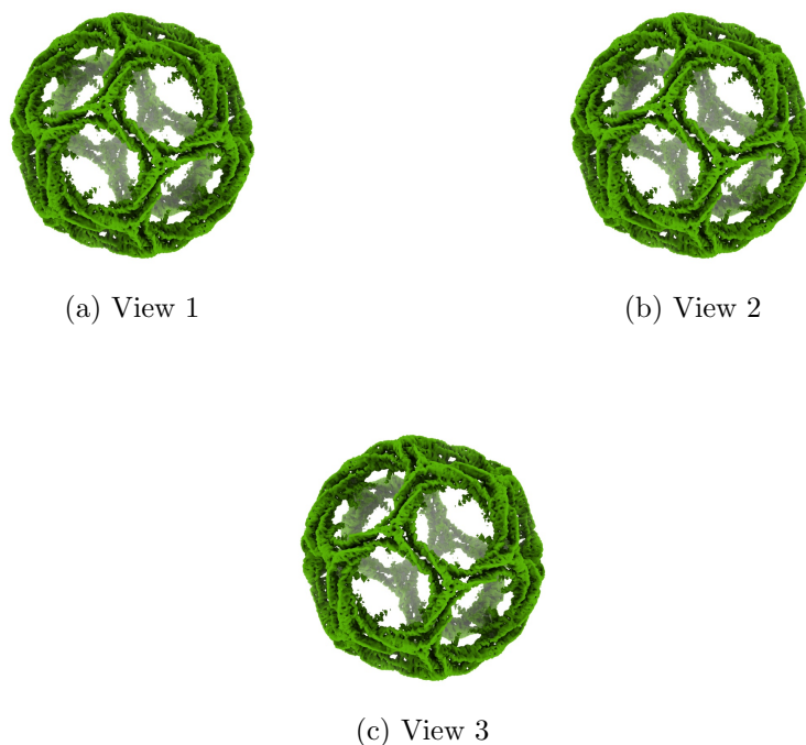
Figure 4: Isosurface at threshold=5.600000. Views generated by ChimeraX at a the following X, Y, Z angles: View 1 (0, -90, -90), View 2 (-90, 0, -90), View 3 (0, 0, 0).
