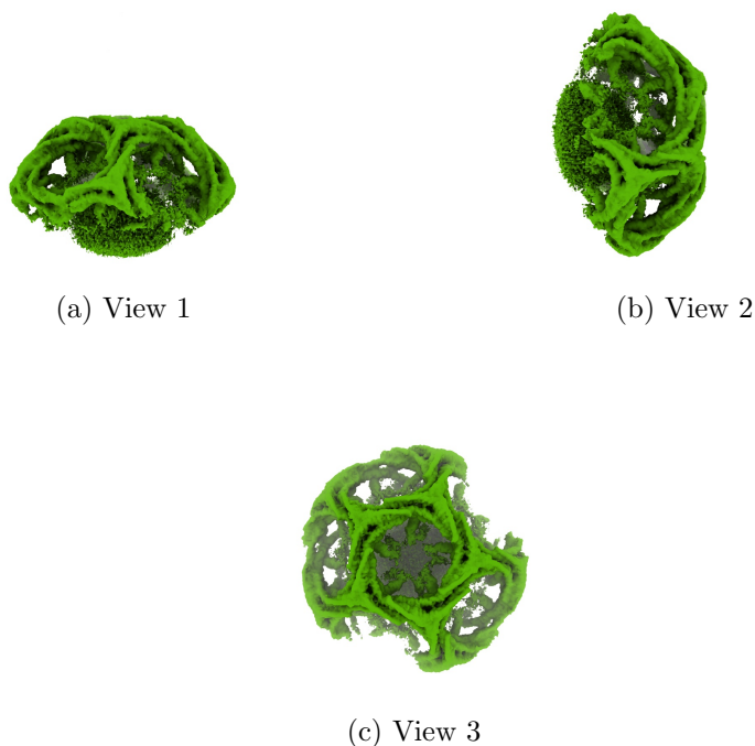
Figure 4: Isosurface at threshold=0.350000. Views generated by ChimeraX at a the following X, Y, Z angles: View 1 (0, -90, -90), View 2 (-90, 0, -90), View 3 (0, 0, 0).
